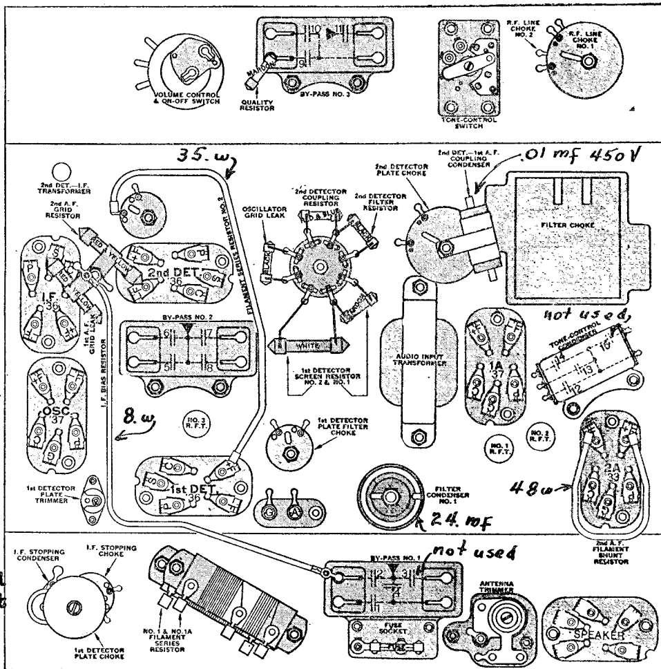
BOTTOM CHART.
